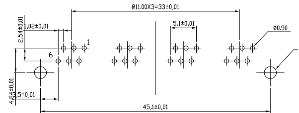
PC Board Layout Component Side Shown
